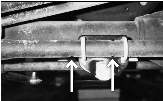
FIG 1 - LOCATING GROOVES
